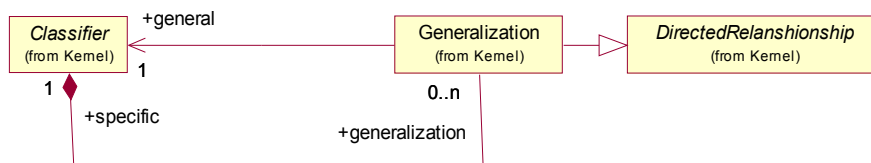
Fig. 2. A part of the UML meta-model -- a relation of the generalization
